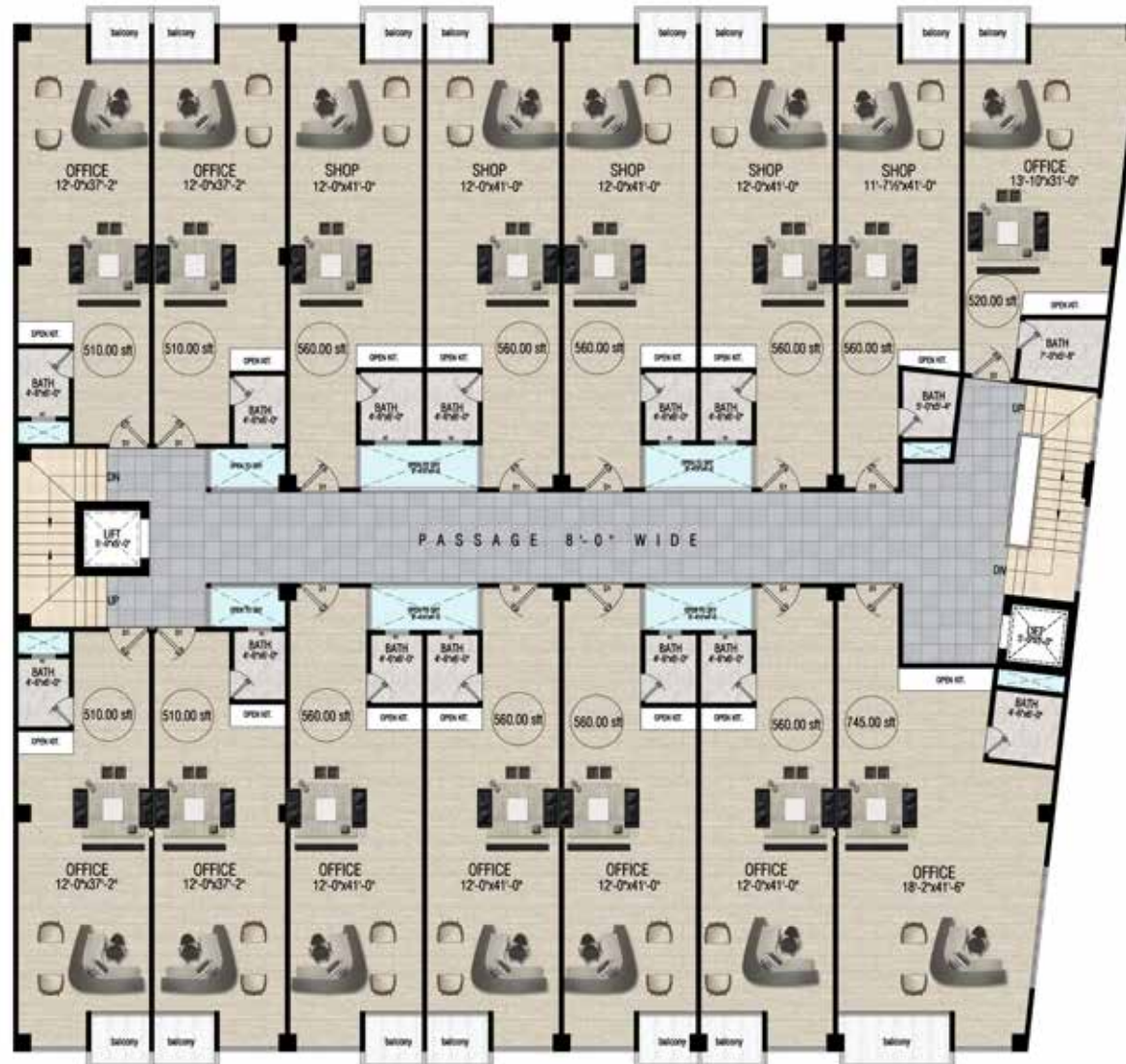
Second to Fifth Floor (Offices)
